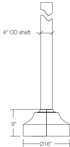
Shown with reducing collar for Ø4" shaft
